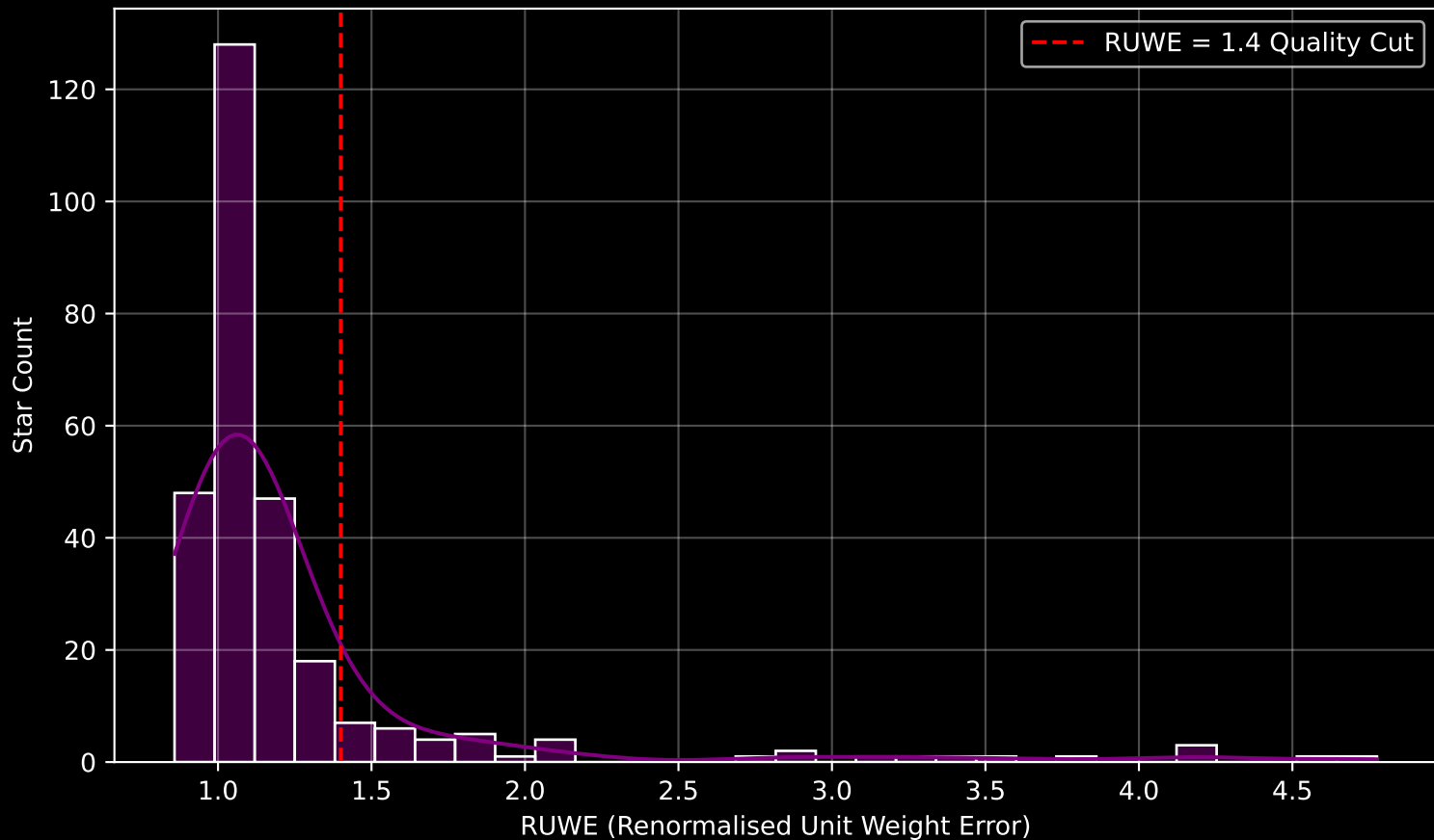
GAPOGEE DR17 Field [ORIONOB1AB-F] RUWE Distribution (n= 281)
