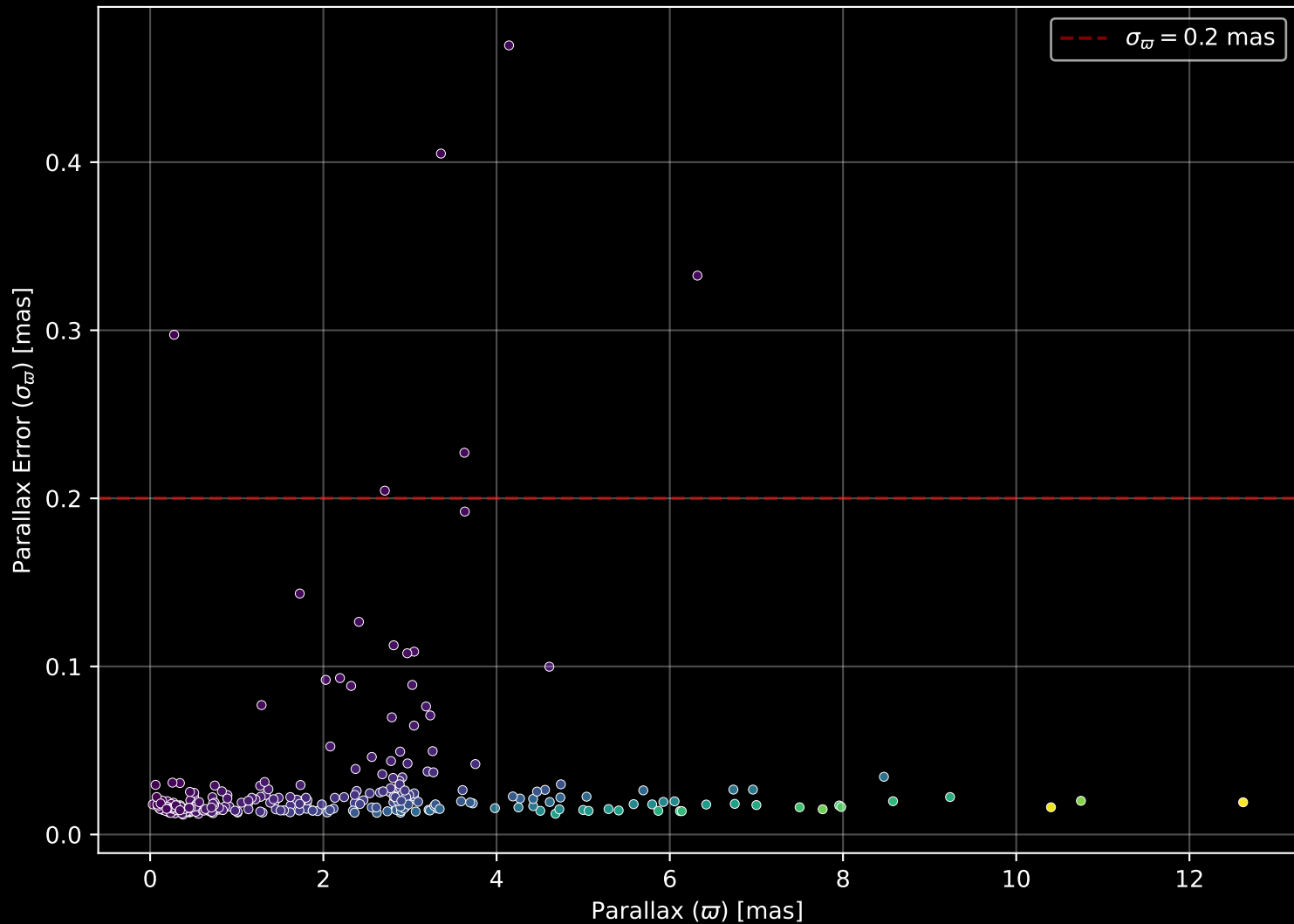
APOGEE DR17 Field: [ORIONOB1AB-F] Parallax Quality (n= 293)
