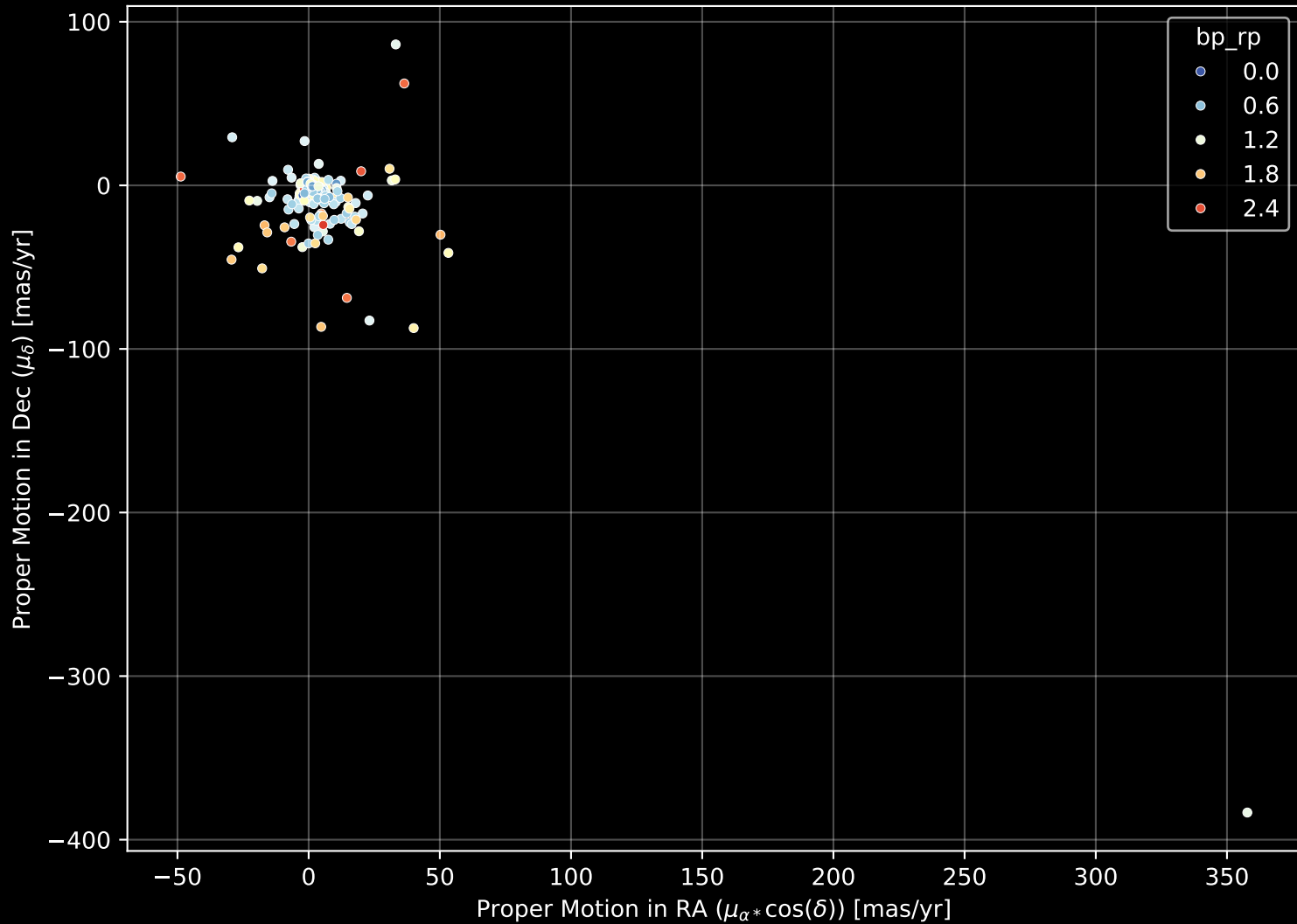
APOGEE DR17 Field: [ORIONOB1AB-F] Proper Motion Diagram (n= 293)
