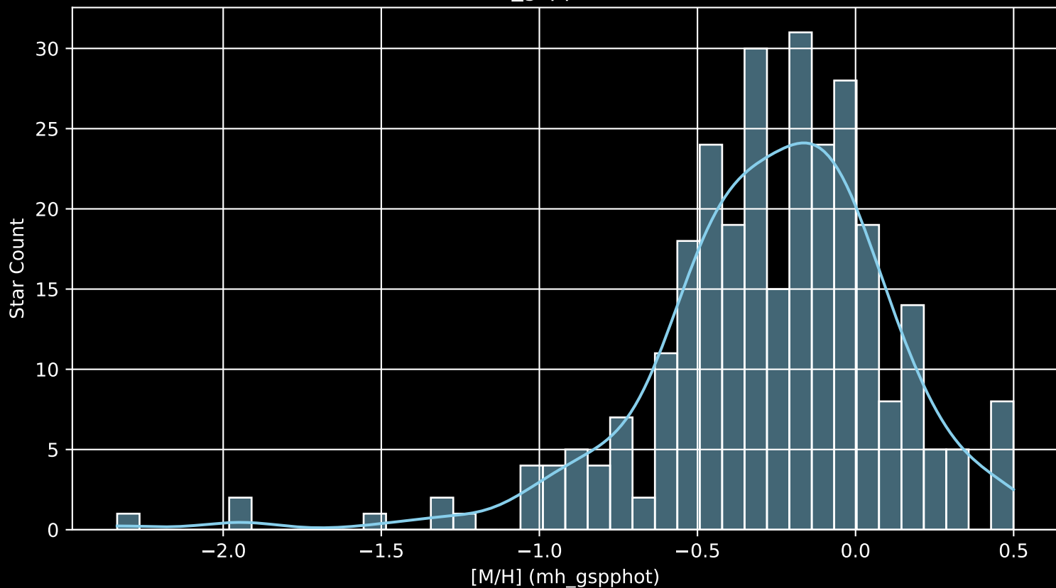
APOGEE DR17 Field: [ORIONOB1AB-F [M/H] (mh_gspphot) (n= 292)
