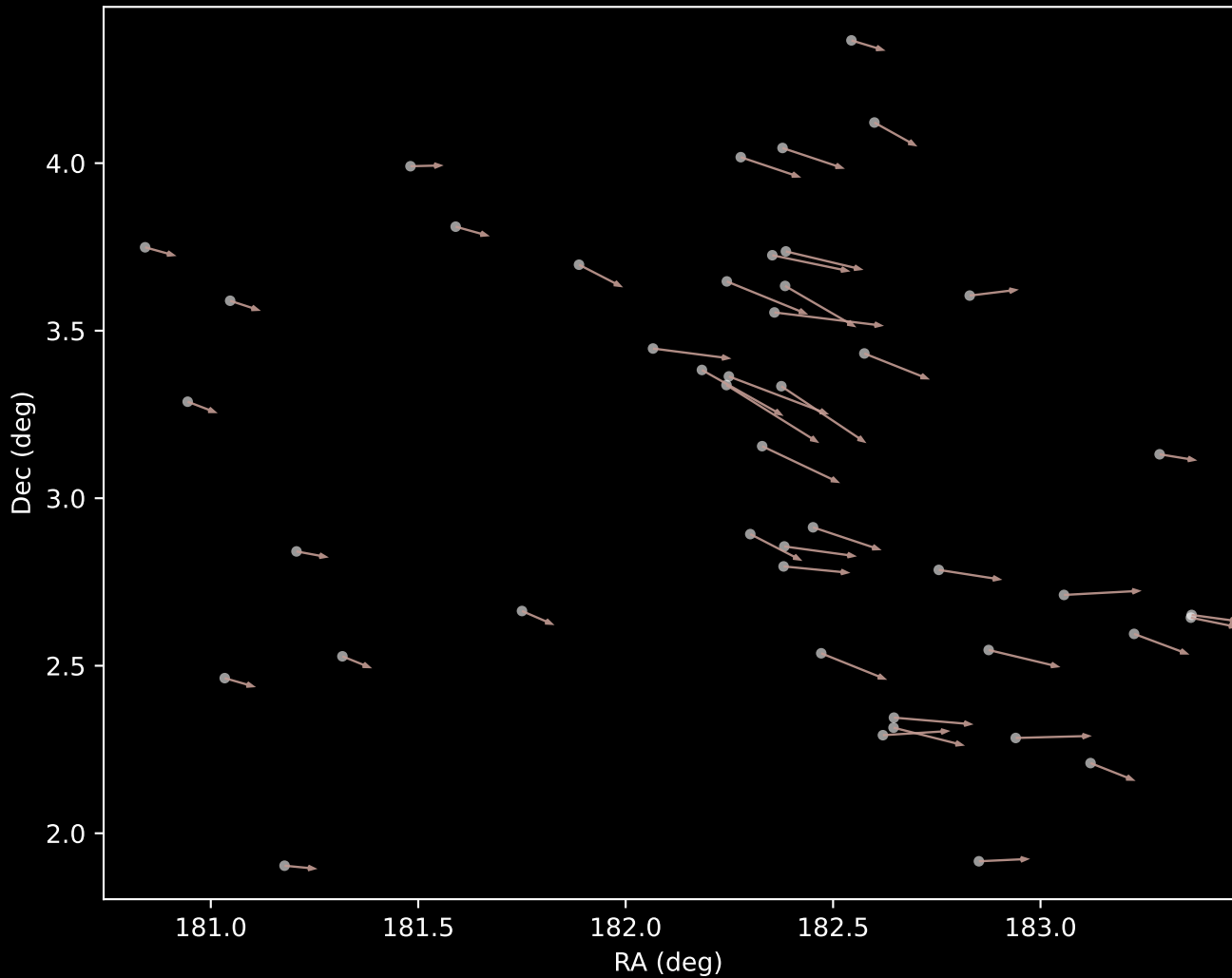
APOGEE DR17 Cluster 11 Proper Motion Vectors (n=46)
