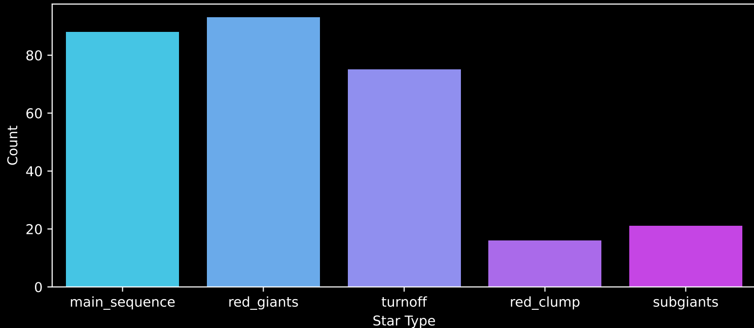
APOGEE DR17 Field: [ORIONOB1AB-F] Count plot of Star Type
