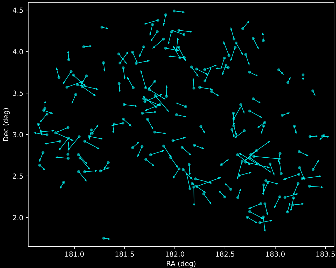
APOGEE DR17 Noise Stream Proper Motion Vectors (n=173)
